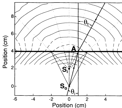
FIG. 3. Constant phase contours (in 20^\circ intervals) as a function of position showing the propagation of a diffuse photon density wave across a planar boundary that separates 1% concentrated Intralipid from 0.25% Intralipid. See text for detailed discussion. S_0 , source position; S_i , apparent source position; A , point on boundary; \theta_i , angle of incident ray; \theta_r , angle of refracted ray. The solid lines are obtained directly from data. The dot-dashed lines are obtained by interpolation over large distances, and are drawn to show the irregularities at large angles.
