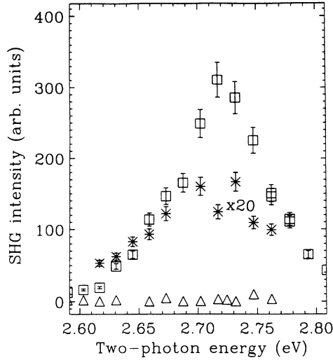
FIG. 8. Variation of SH intensity as a function of two-photon energy in the s -in/ s -out ( \triangle ) and s -in/ p -out ( * ) polarization configurations. The interfacial SH spectrum ( \square ) is shown for comparison. The s -in/ s -out intensity is below our detection limit and the s -in/ p -out peak intensity is \sim 40 times smaller than the interface signal.
