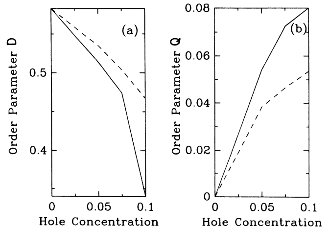
FIG. 2. Variation of the order parameters D and Q with the hole concentration \delta . (a) shows variation in D for t_2=0 (solid line) and t_2=0.5 (dashed line). (b) shows variation of Q for the same two values of t_2 .
