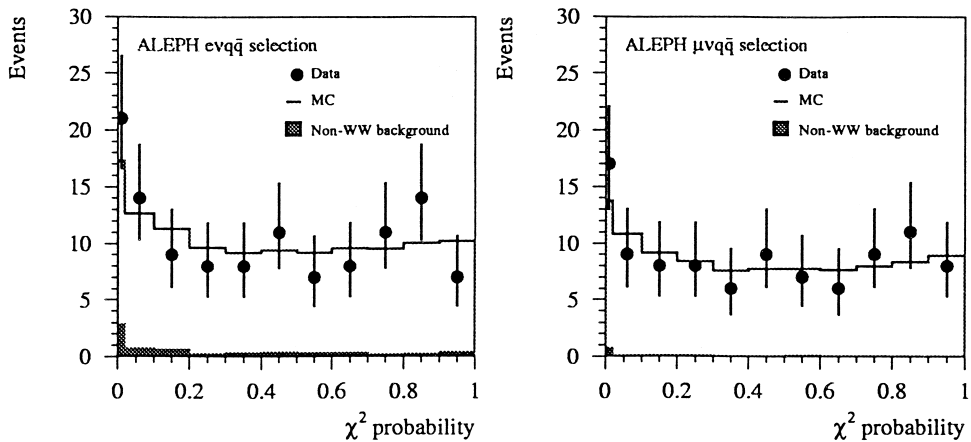
Fig. 1. The \chi^2 probability distribution for 2C kinematic fits in the e and \mu channels.
