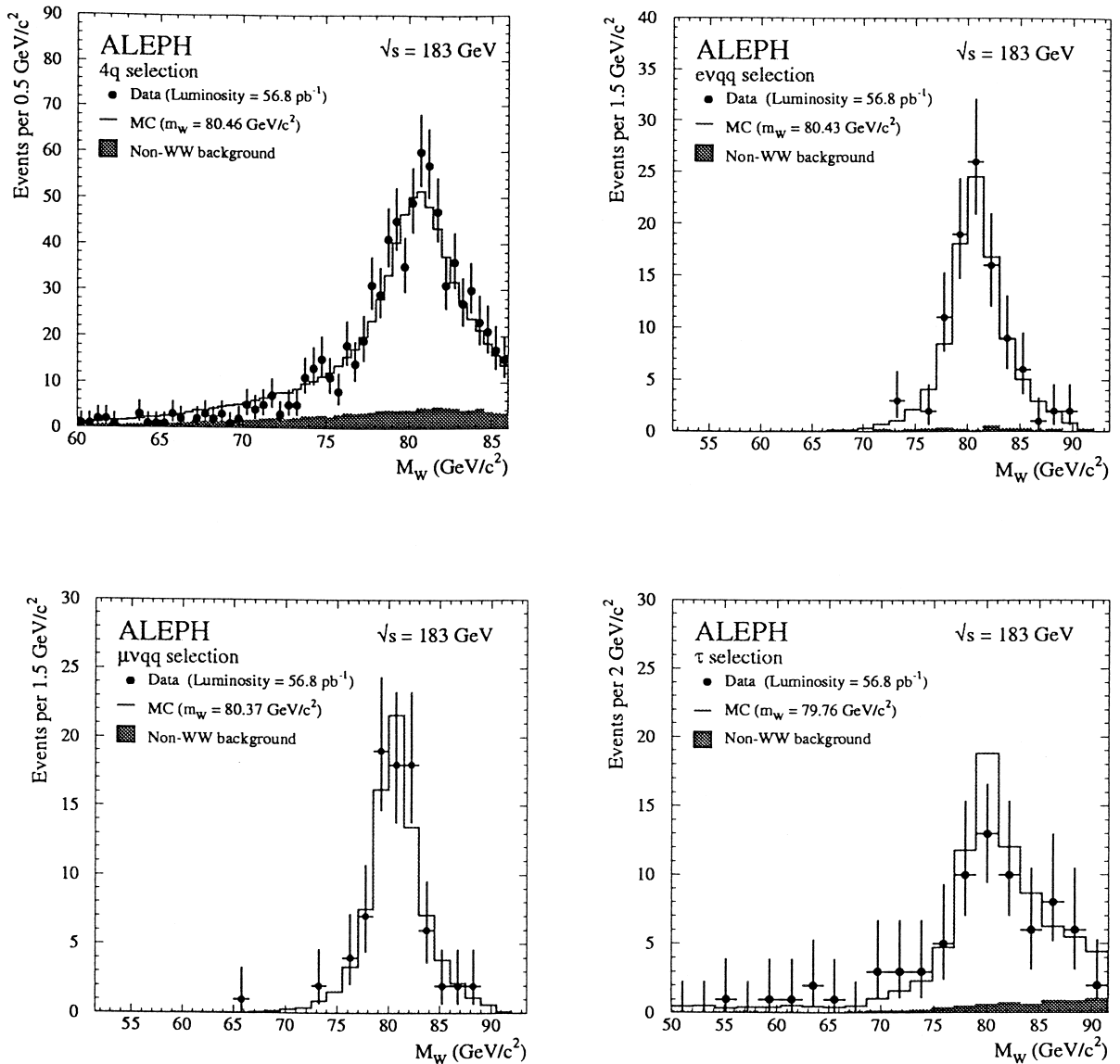
Fig. 2. (a),(b),(c) and (d) Mass distributions for the 4q, e, \mu , and \tau data (points with error bars), non-WW background (shaded area) and signal + background Monte Carlo with m_W values as quoted (solid line histogram).
